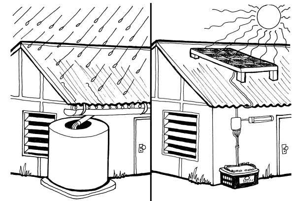
Rainwater system. Photovoltaic system.
