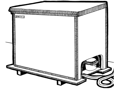
A typical vaccine refrigerator with top-opening lid, external batteries and the compressor and condenser in the main housing.
